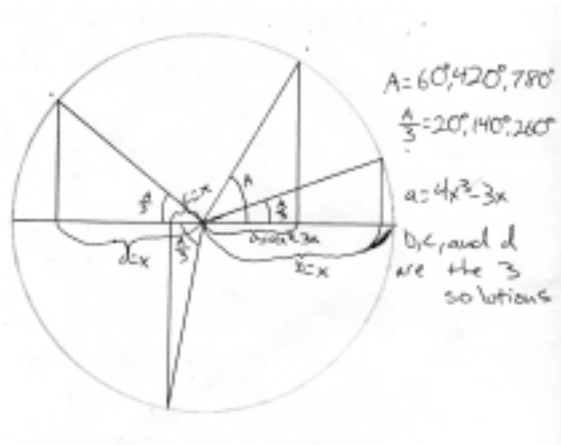
Three solutions to cubic function in the complex domain: Tripling the angle of any of the three solutions of 20°, 140°, and 260° will bring you to the desired 60°.
