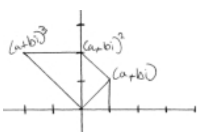
Cubing a complex magnitude (a + bi)\sqrt{-1} in the complex domain, a combination of rotation and extension.
