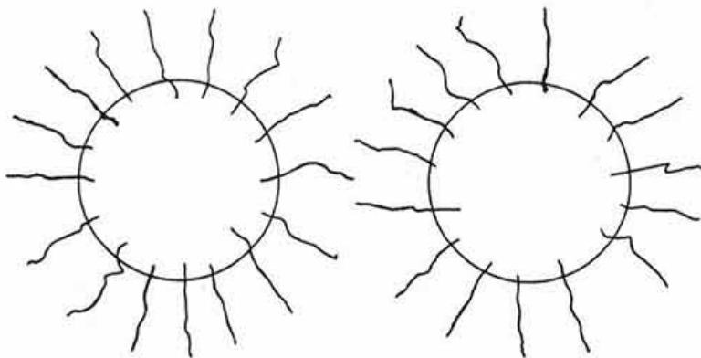
METHOD 3: Steric hindrance due to adsorption of an oriented nonionic polyelectrolyte
