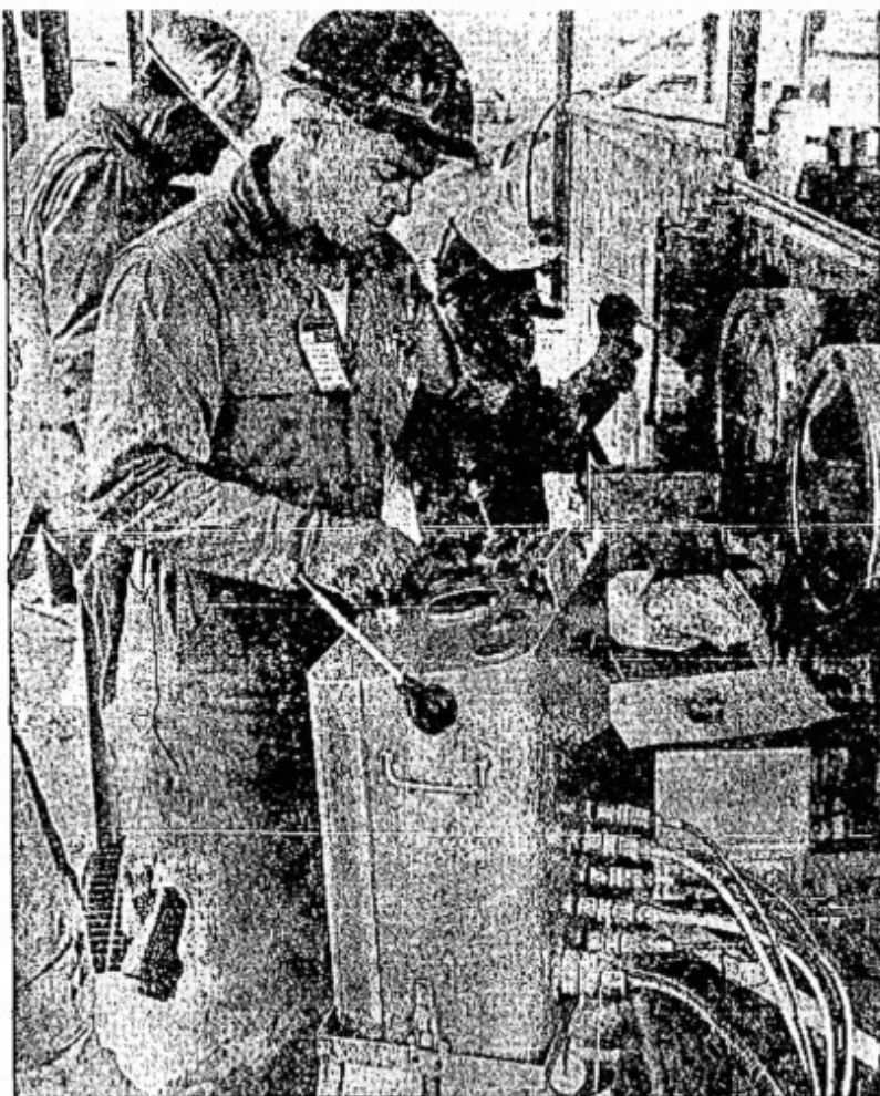
NO OIL FIELD, THIS —Working behind shielding, Halliburton Co. personnel use dismantled oil field service units to dispose of radioactive waste at Oak Ridge nuclear site. The disposal process is based on two oil field techniques—cementing and fracturing.
